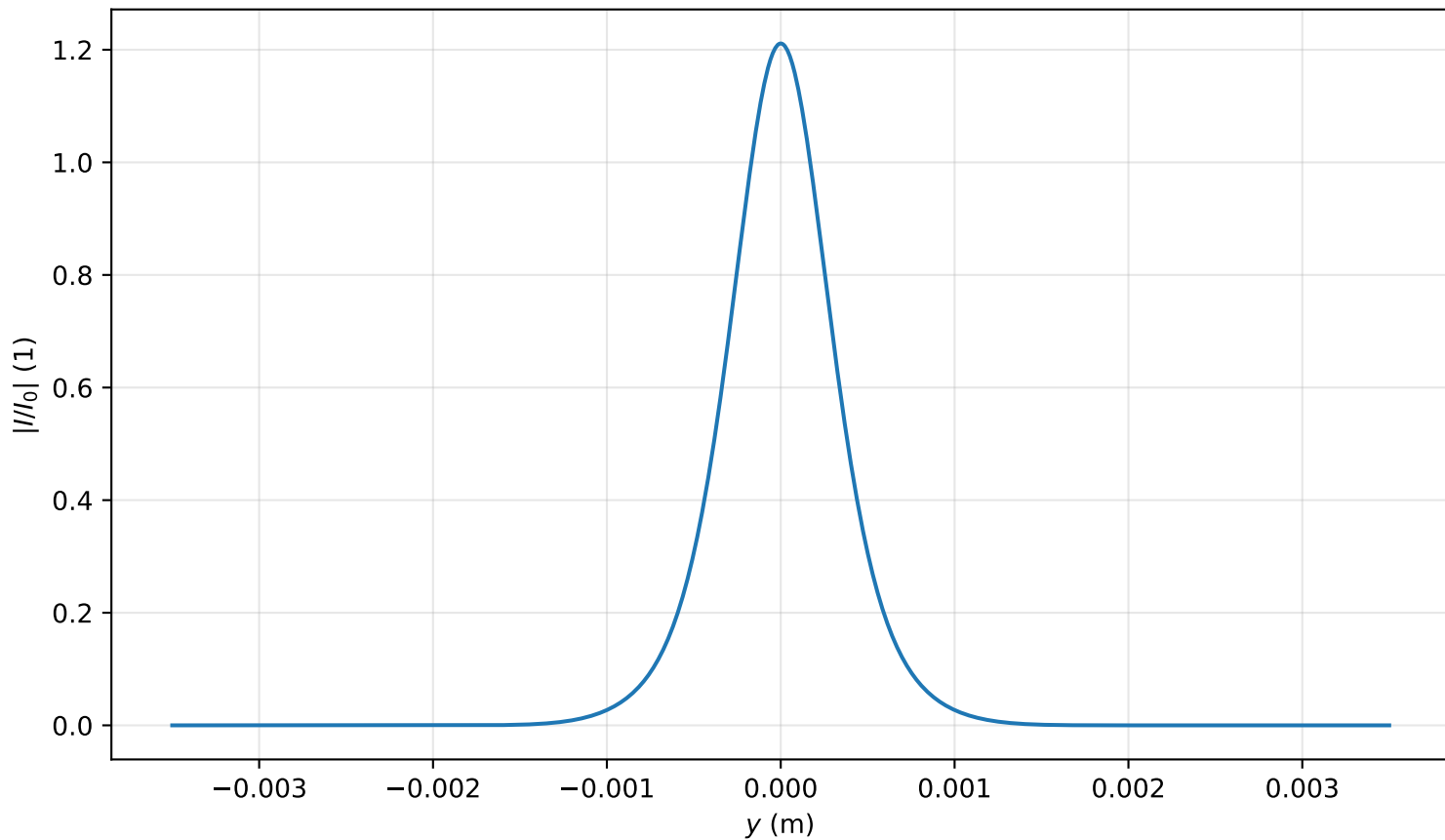
Intensity profile I(x=0, y, z=1.274)/I_0 , P_{in}=0.7P_{cr} , artificial time
